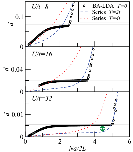
FIG. 4. (Color online) The circles and solid line show the same as Fig. 3 but for three values of U . The dashed (dotted) lines show results computed from an exact second-order high-temperature series expansion at T = 2t ( T = 4t ). The plateau at finite d indicates strong quantum fluctuations. The double arrow in the bottom panel indicates the observable effects of weak thermal fluctuations in a trap and corresponds to the double arrow in Fig. 1.
