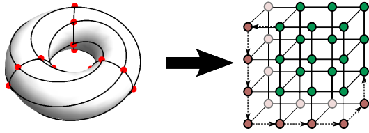
FIG. 1 (color online). An embedding of the toric code into a cubic lattice. Twisted-periodic boundary conditions are imposed by SWAP-gate shuttling along auxiliary sites, indicated by dashed arrows. Bold lines connect logical nearest neighbors [18].
